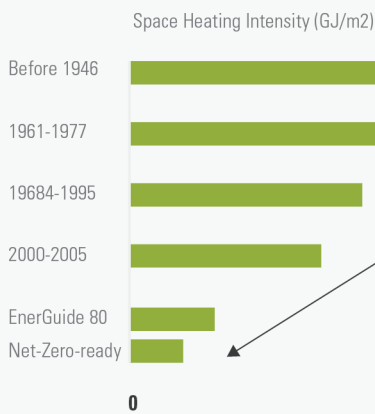
Figure 24 Residential Building Space Heating Intensity by Vintage (Ontario)
