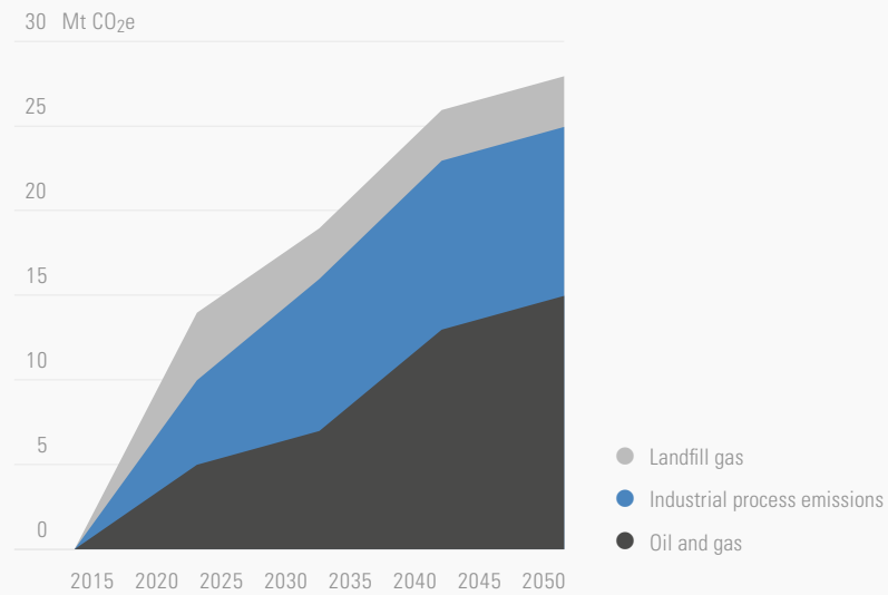
Figure 29 Abatement of fugitive and industrial process emissions
